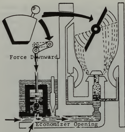
FIGURE 3-13. Accelerating system.
